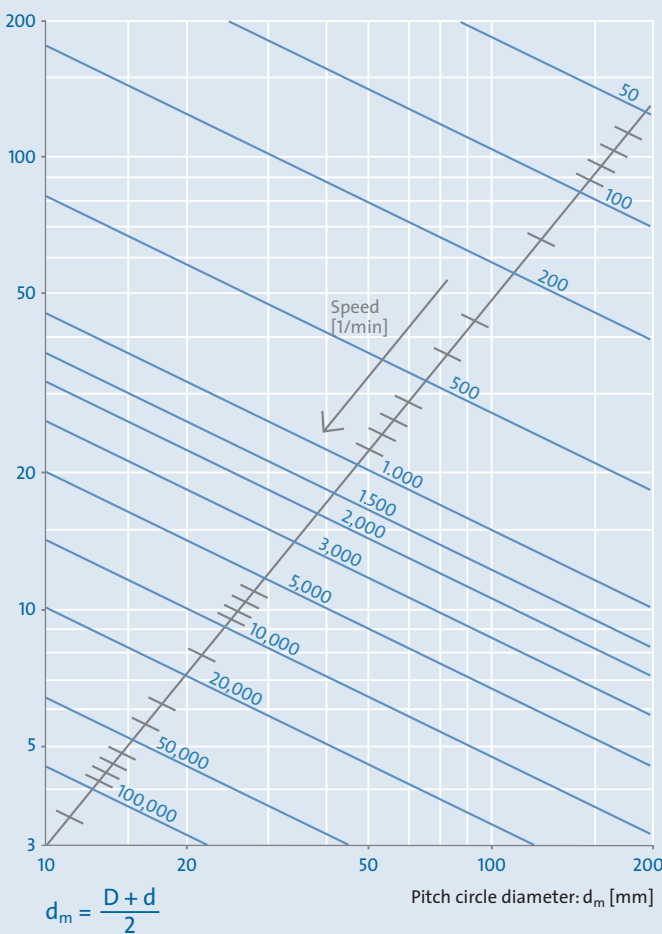
Operating viscosity v_1 [mm 2 /s]
