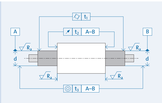
Guidelines for shaft and housing fits / shape and position tolerances (DIN EN ISO 1101)
